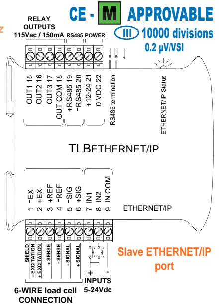
MORSETTIERE ESTRAIBILE EXTRACTABLE TERMINAL BOARDS
